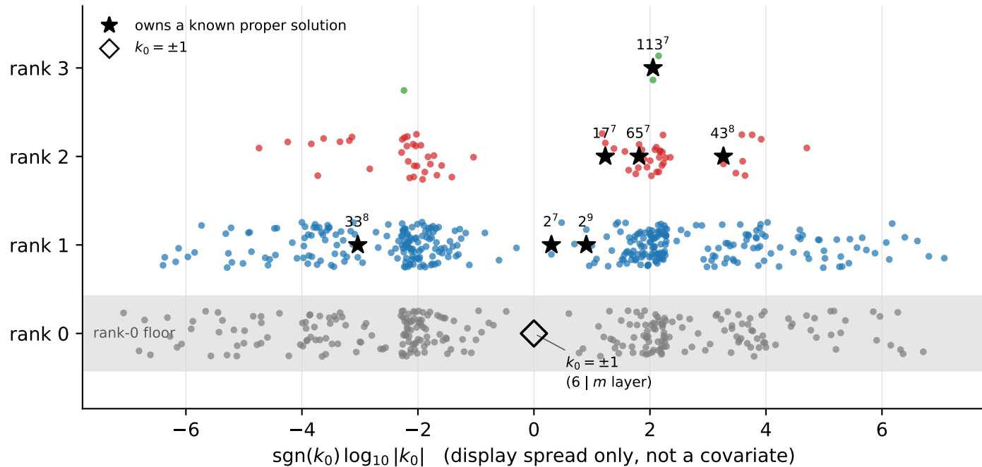
(a) the 670 sixth-power-free classes, by Mordell-Weil rank
