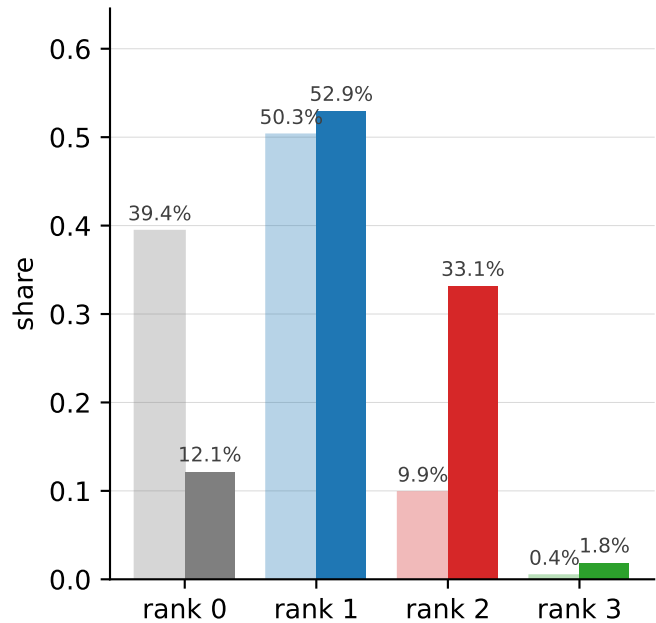
(b) share of classes (pale) against share of E(1000) diagnostic mass (solid)
