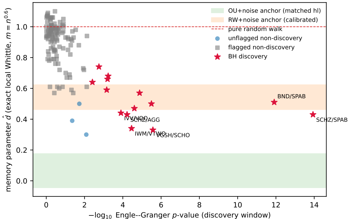
Fractional integration census of all 130 spreads
