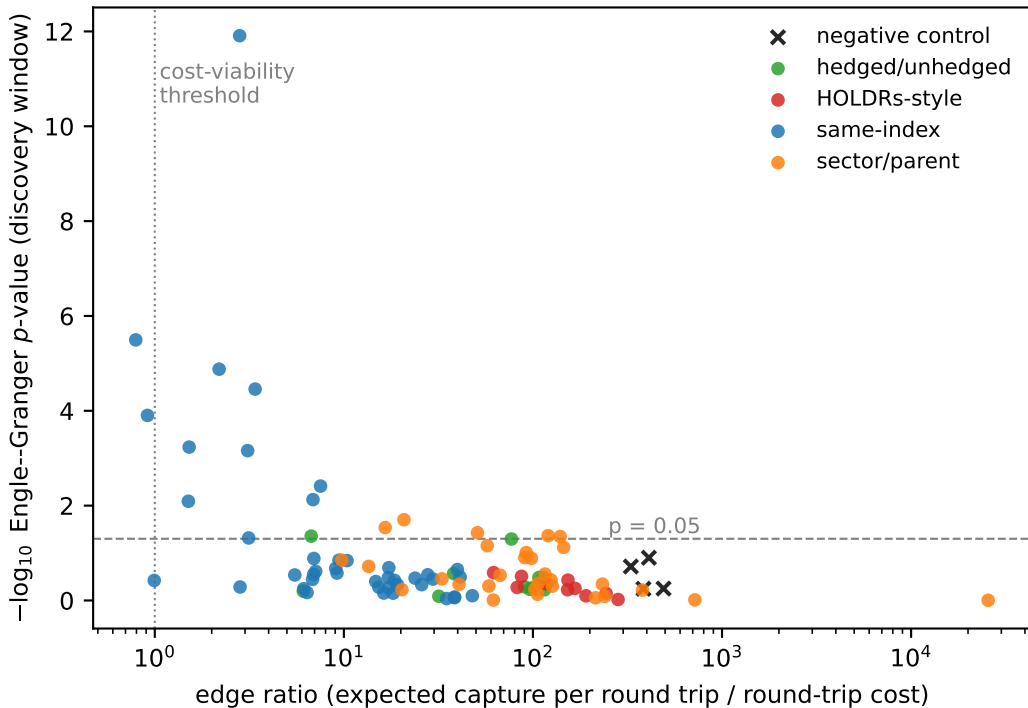
Cointegration strength vs. cost viability, 98 ETF pairs
