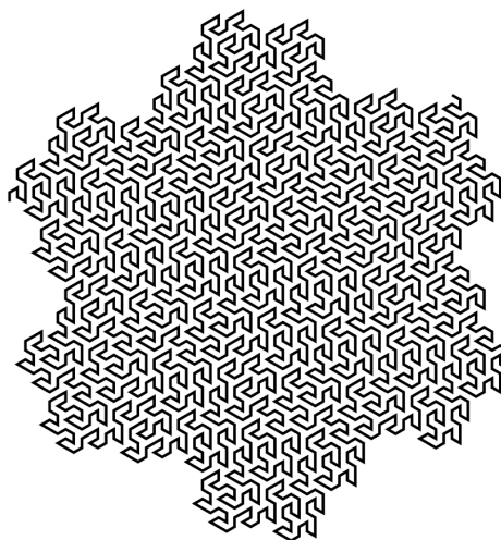
(b) Gosper-Kurve
