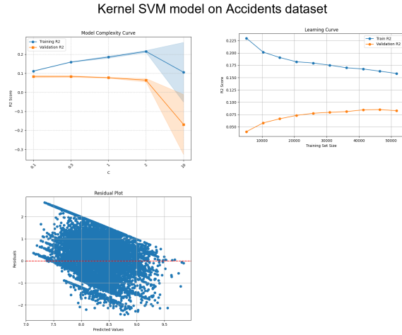
Fig. 6. All Graphs for Kernel SVM (Accidents Dataset)
