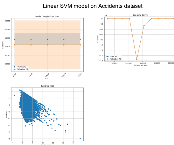
Fig. 11. All Graphs for Linear SVM (Accidents Dataset)
