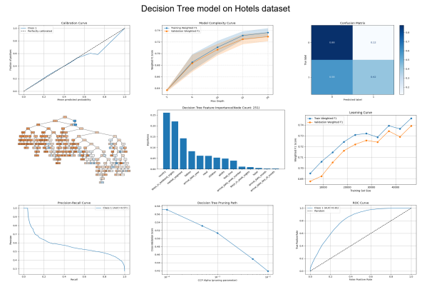
Fig. 1. All Graphs for Decision Tree (Hotels Dataset)
