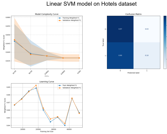
Fig. 10. All Graphs for Linear SVM (Hotels Dataset)
