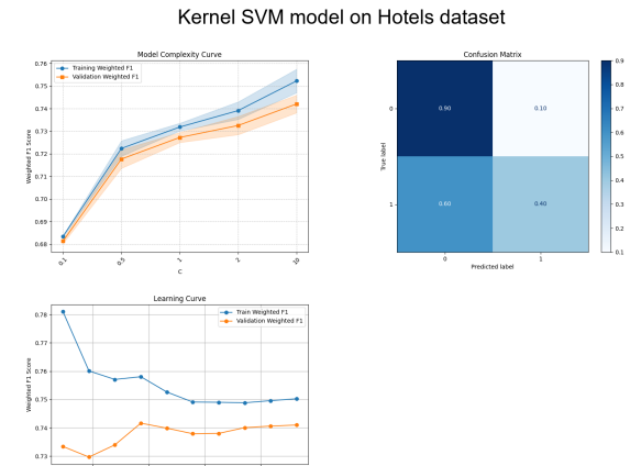
Fig. 5. All Graphs for Kernel SVM (Hotels Dataset)
