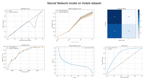
Fig. 7. All Graphs for Neural Network (Hotels Dataset)
