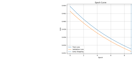
Fig. 8. All General Epoch curves for all Neural Networks (plotted using Hotels)
