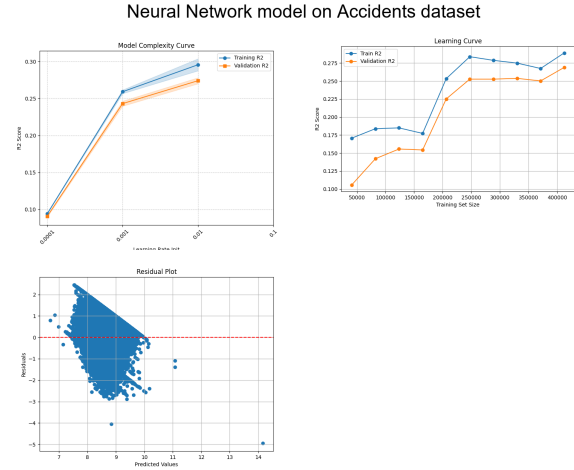
Fig. 9. All Graphs for Neural Network (Accidents Dataset)
