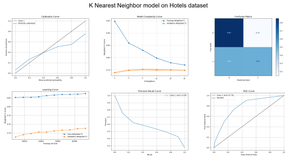
Fig. 3. All Graphs for K-Nearest Neighbor (Hotels Dataset)
