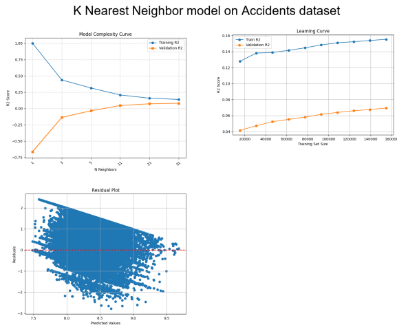
Fig. 4. All Graphs for K-Nearest Neighbor (Accidents Dataset)
