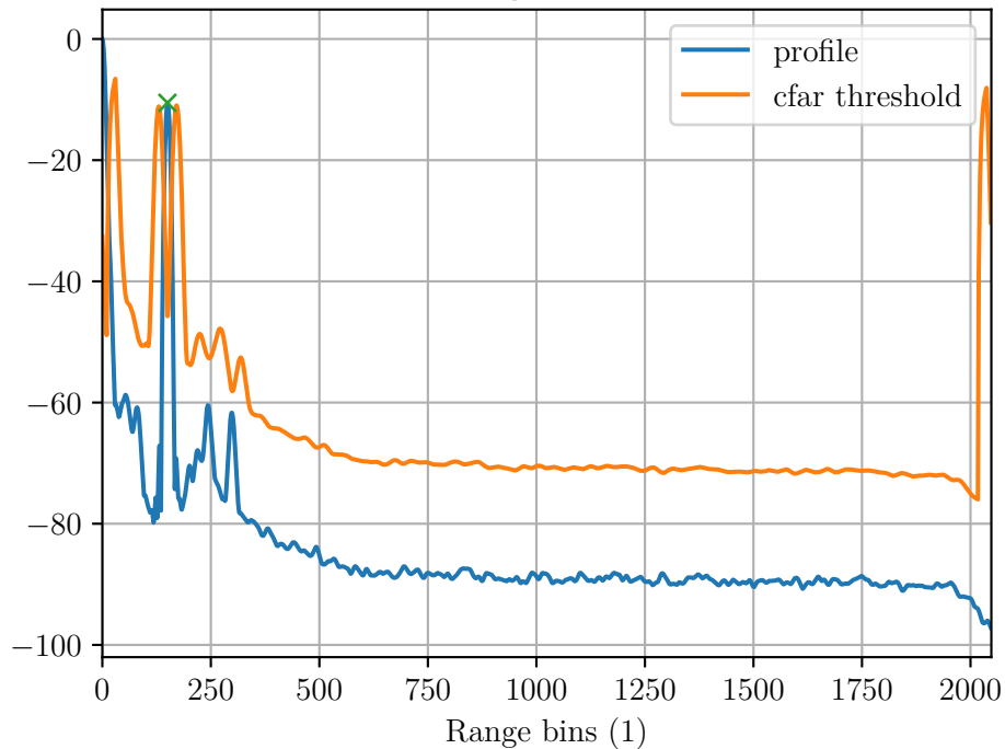
Range profile
