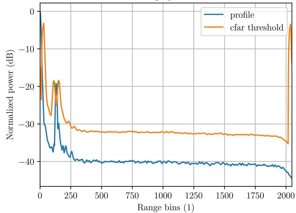
Range profile
