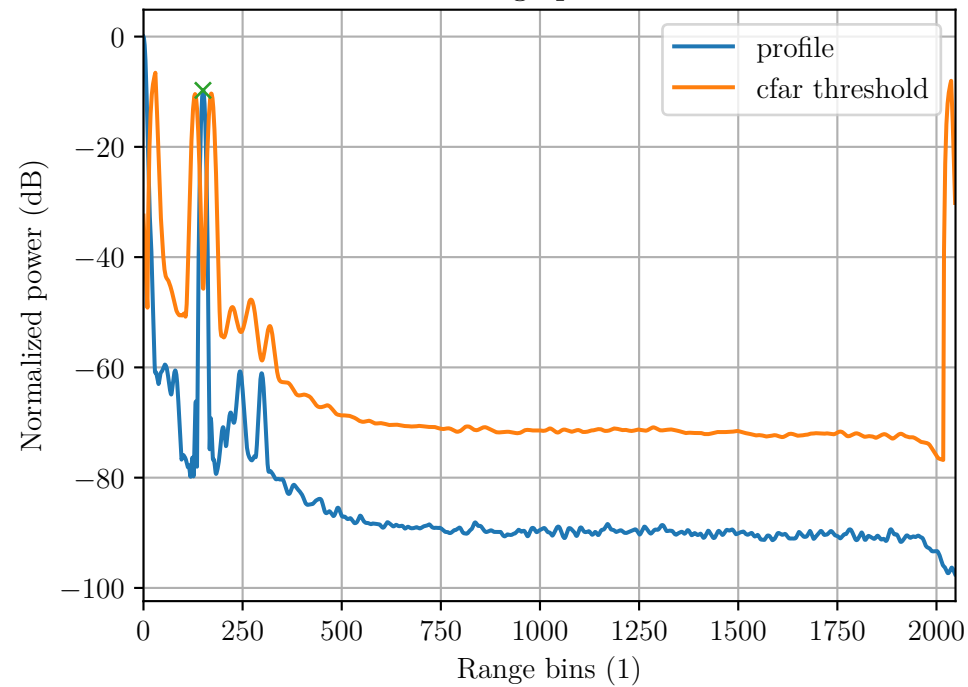
Range profile
