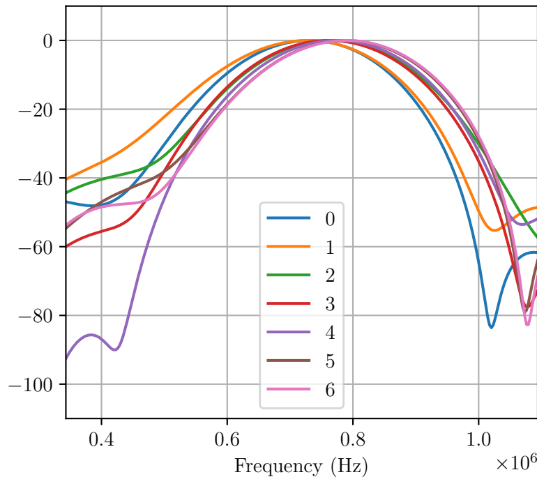
Blockwise Chirp z-Transformation
