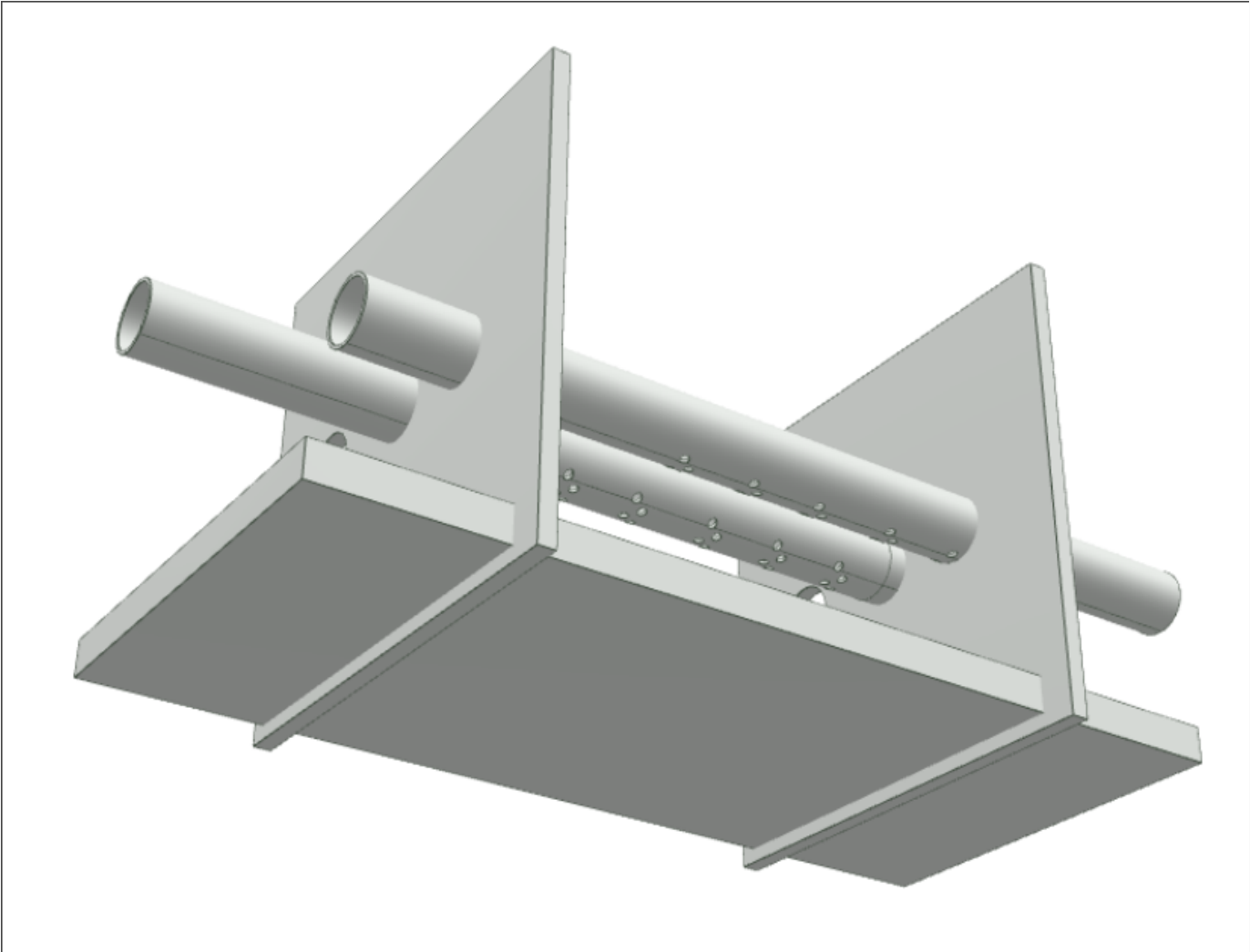
Figure 2: Multicomponent Muffler Internal Geometry
