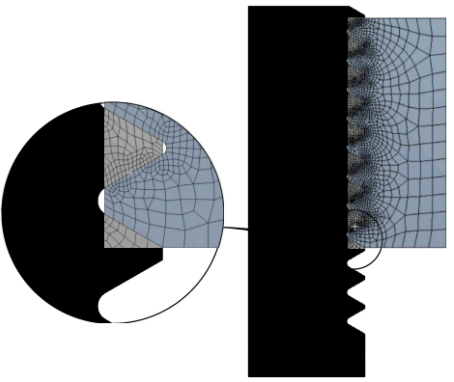
Figure 17: Mesh
