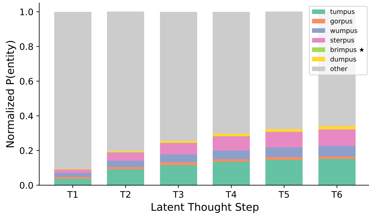
Coconut (Latent)
