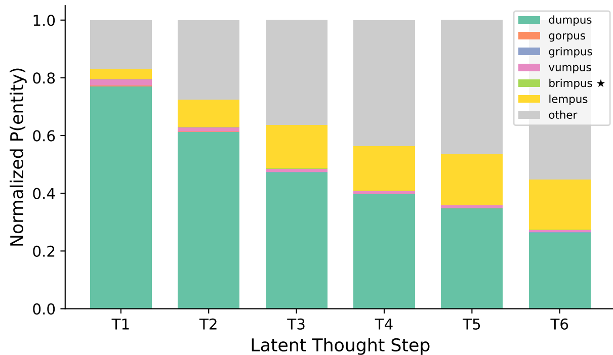
Coconut (Latent)
