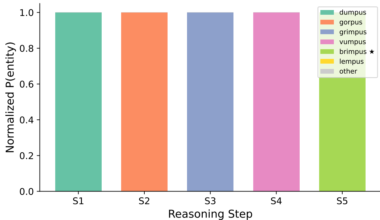
CoT (Discrete)
