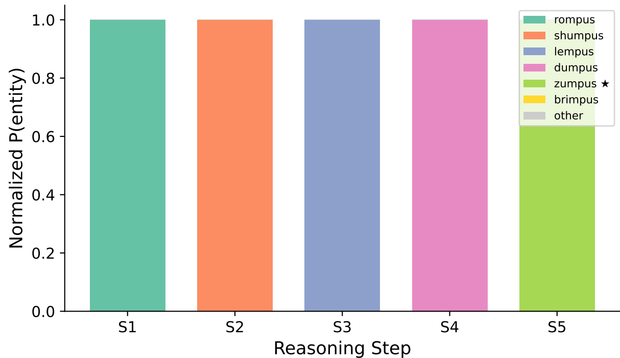
CoT (Discrete)
