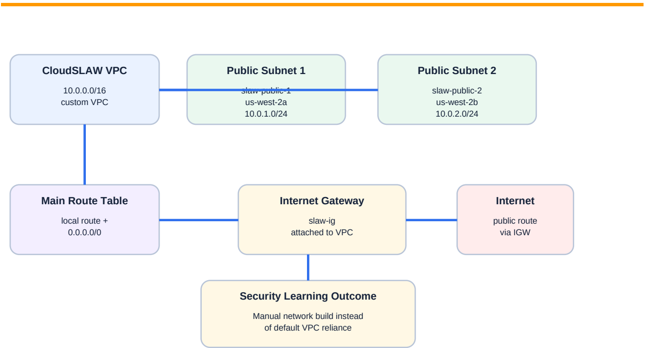
Figure 1 - Custom VPC with two public subnets, route table, and Internet Gateway.
