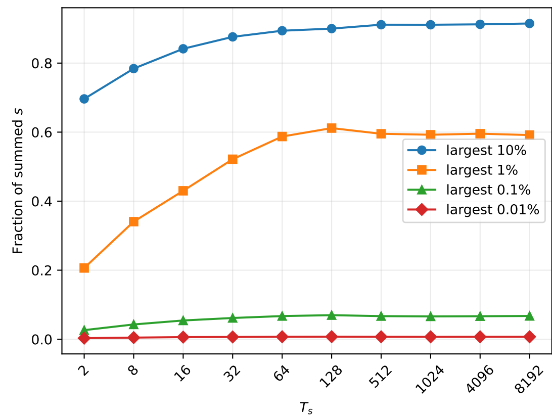
Empirical two-scale partition
