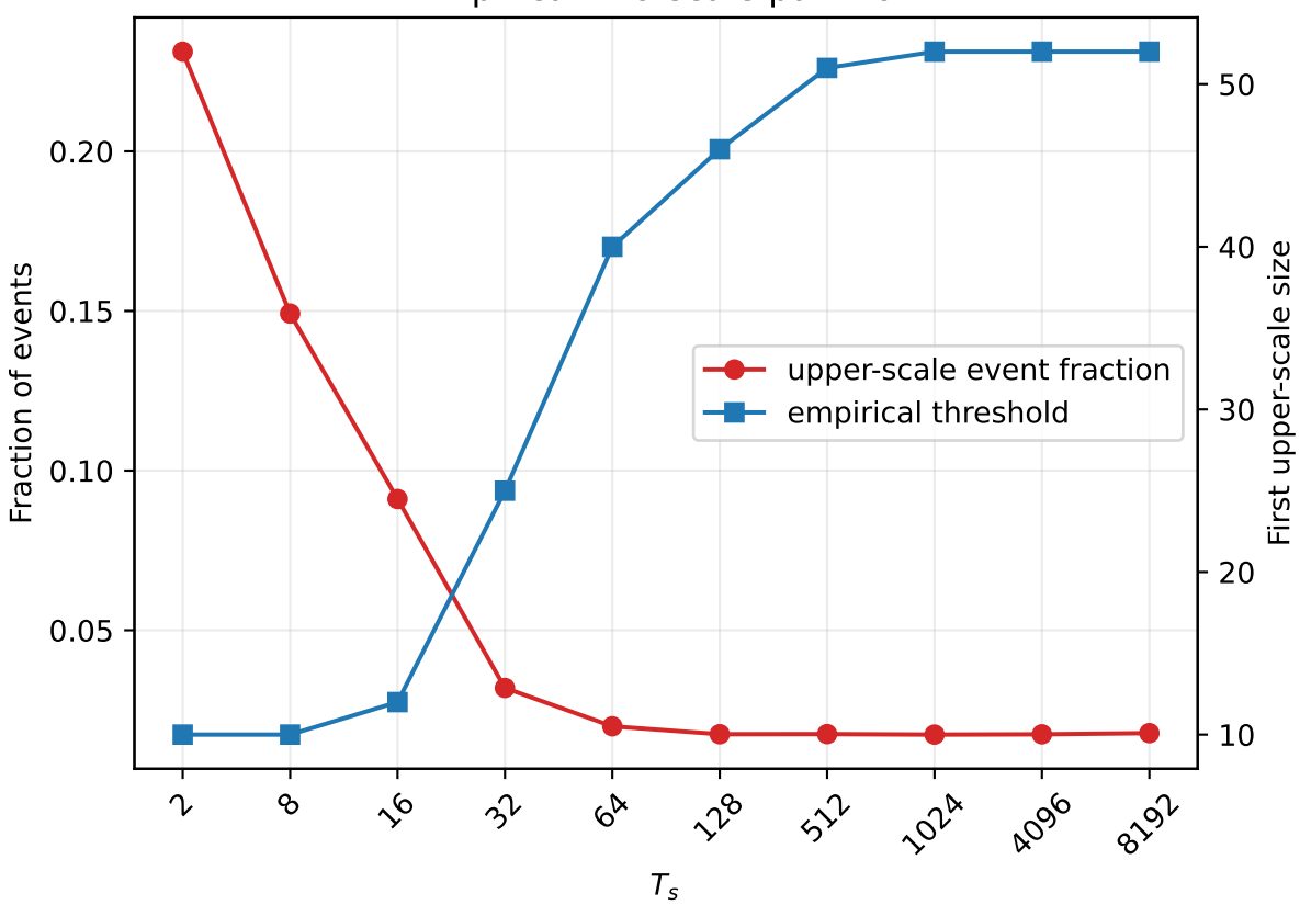
Empirical two-scale partition
