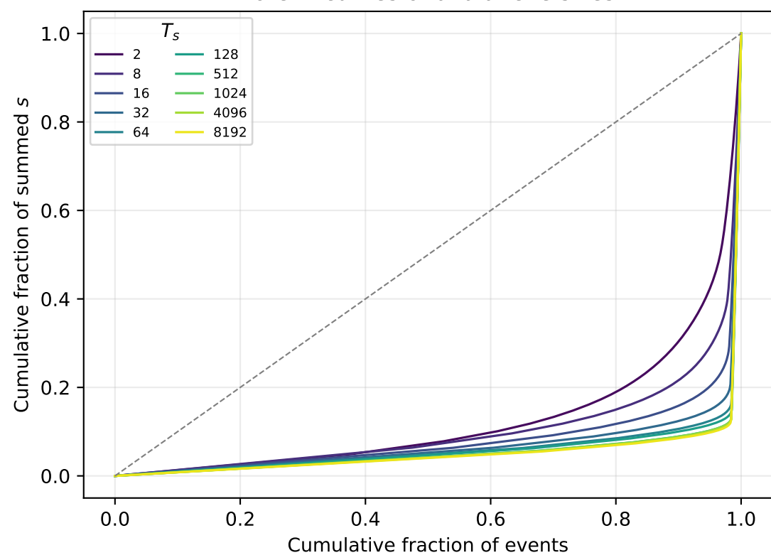
Lorenz curves of avalanche sizes
