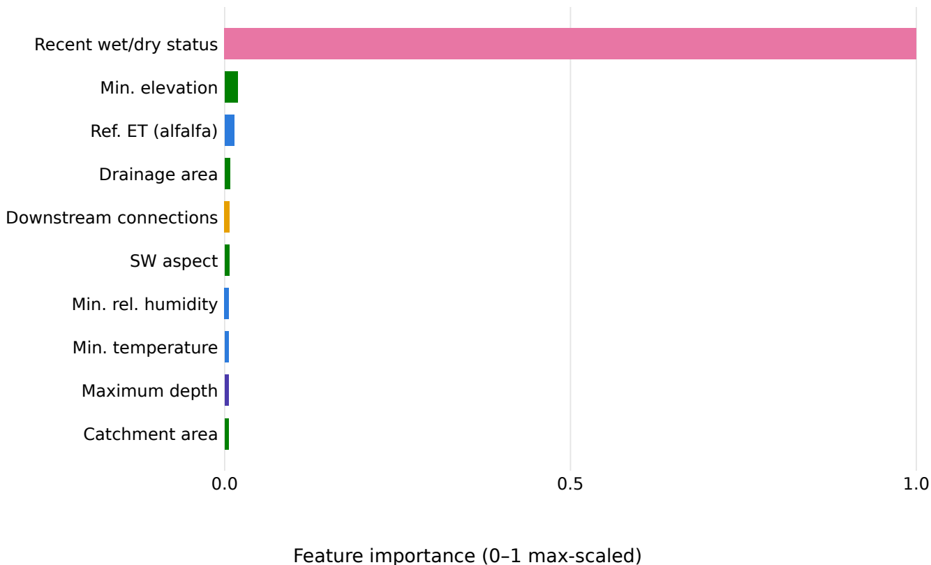
(b) XGBoost gain-based importance
