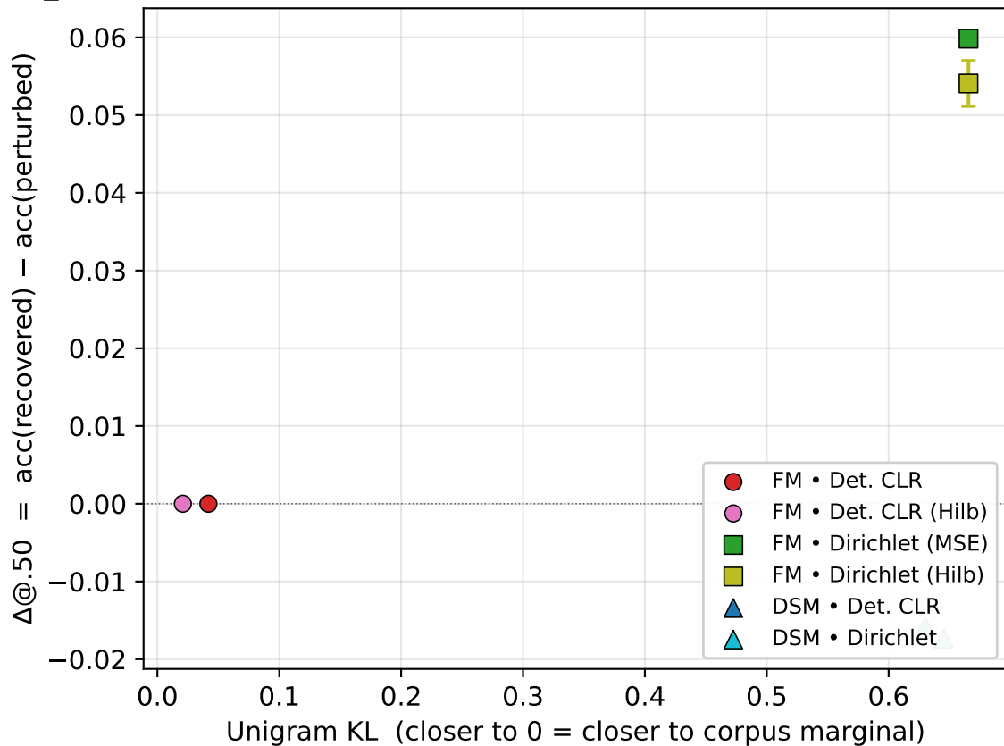
Figure 2 — KL_uni and recovery are decoupled
