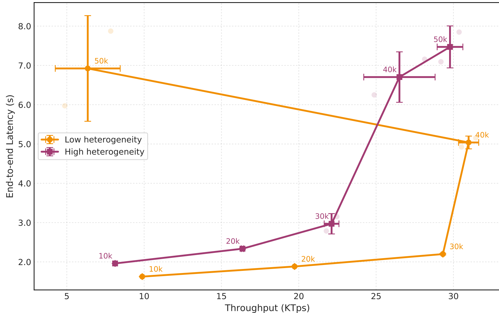
End-to-end Latency vs Throughput
