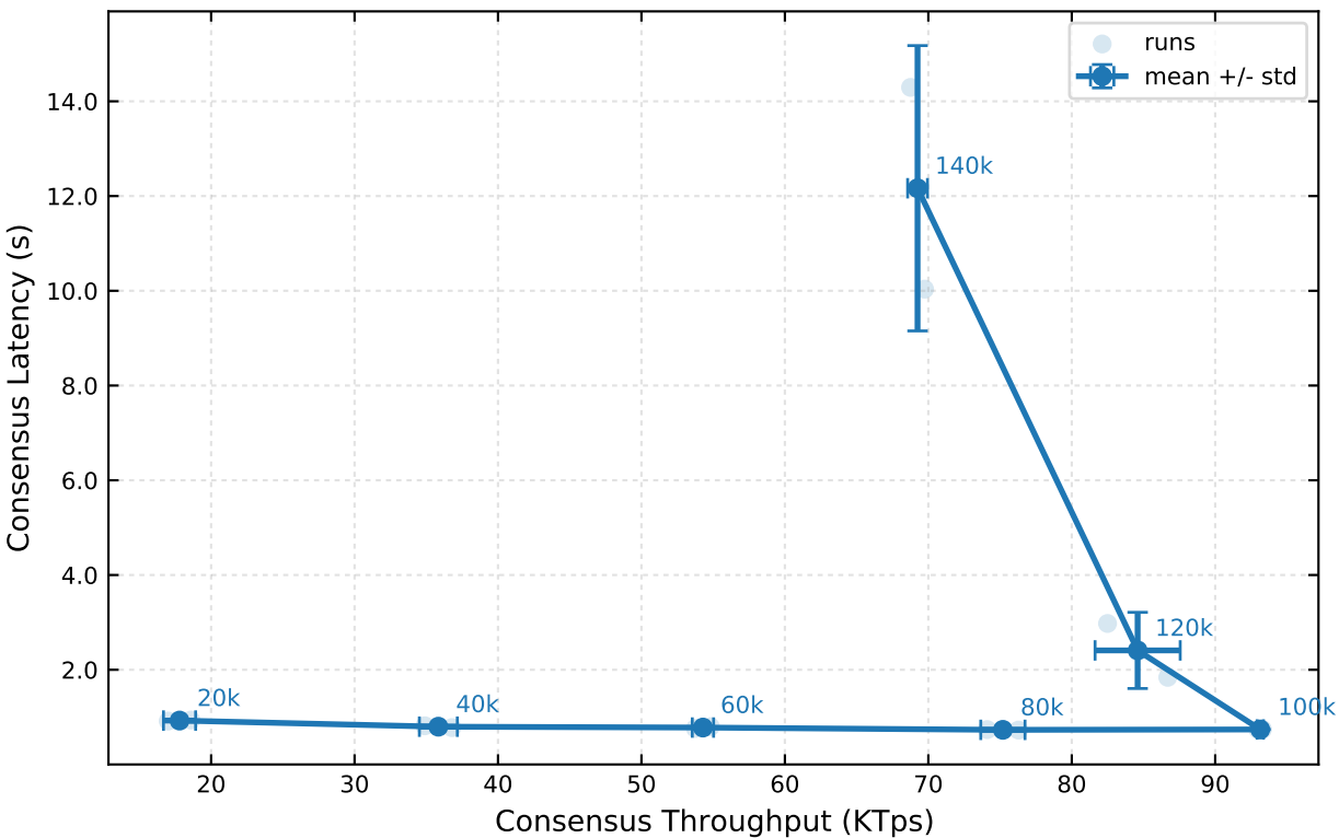
80ms/custom-high-3 Consensus TPS-Latency
