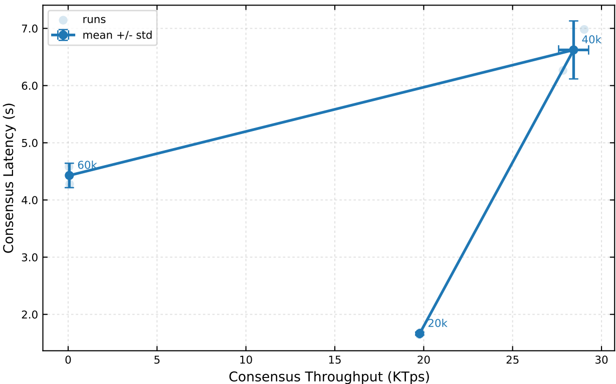
80ms/old/custom-high-3 Consensus TPS-Latency
