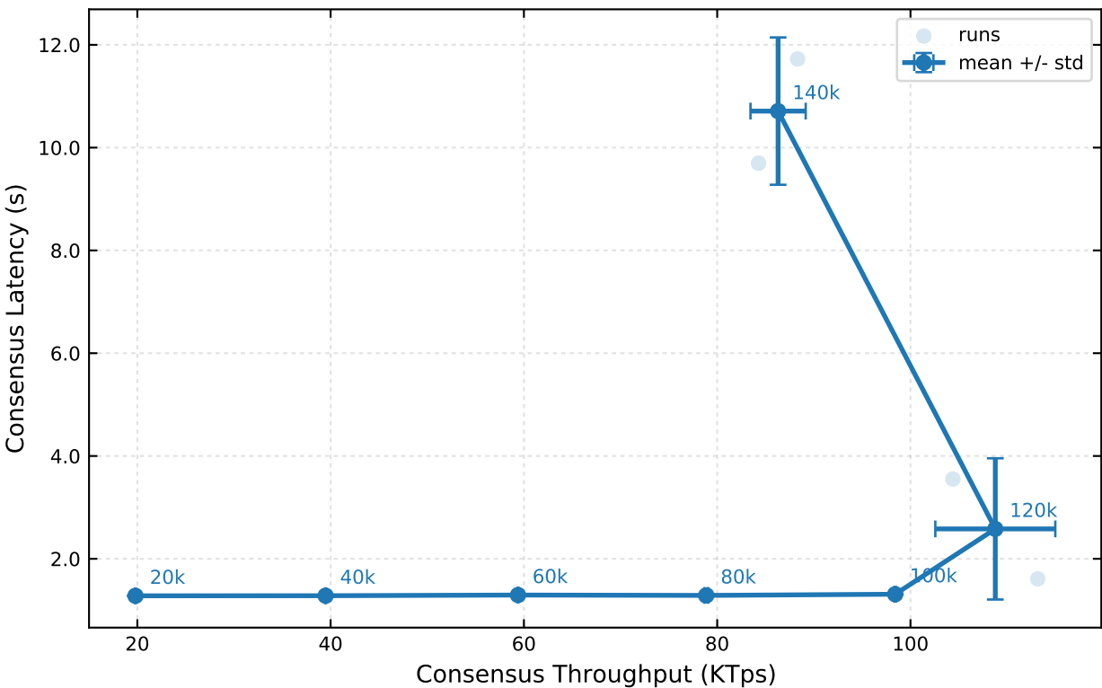
80ms/old/custom-high-5 Consensus TPS-Latency
