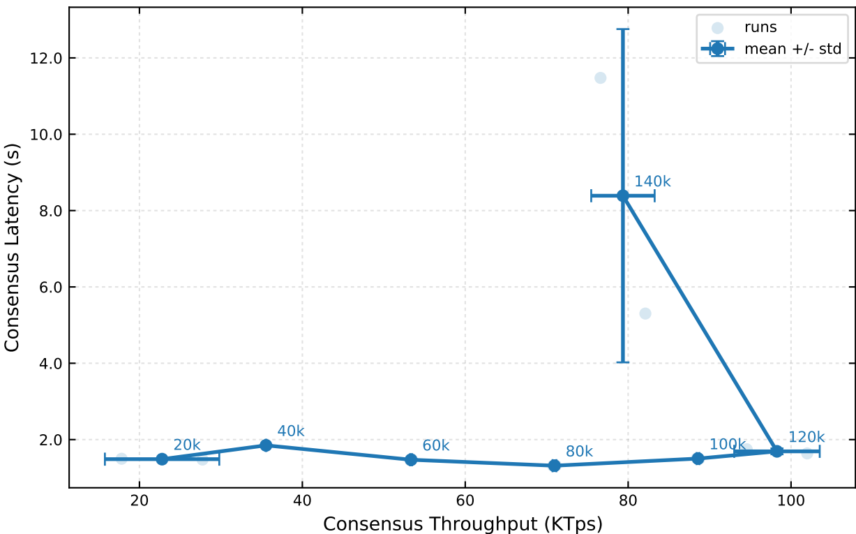
geo/balanced Consensus TPS-Latency
