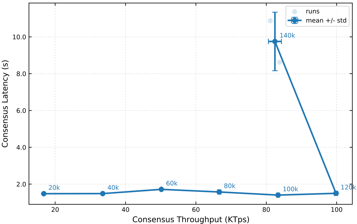
geo/custom-high-3 Consensus TPS-Latency
