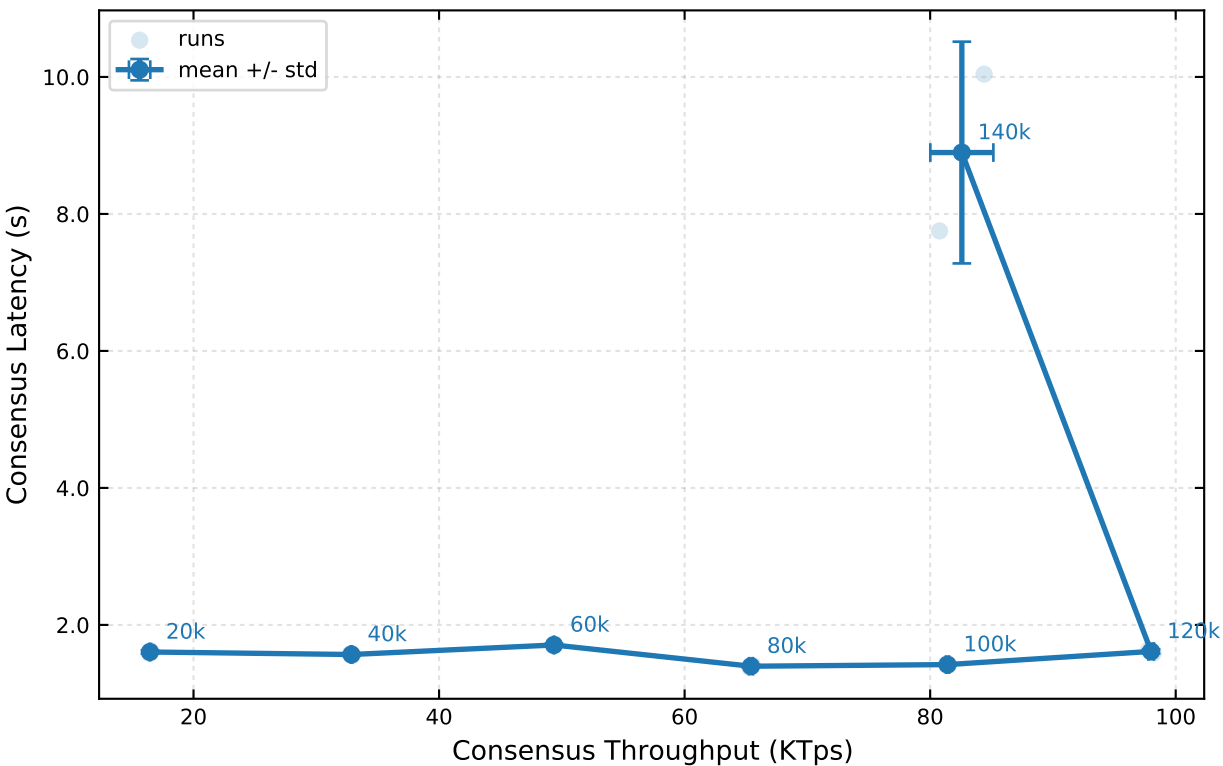
geo/custom-high-5 Consensus TPS-Latency
