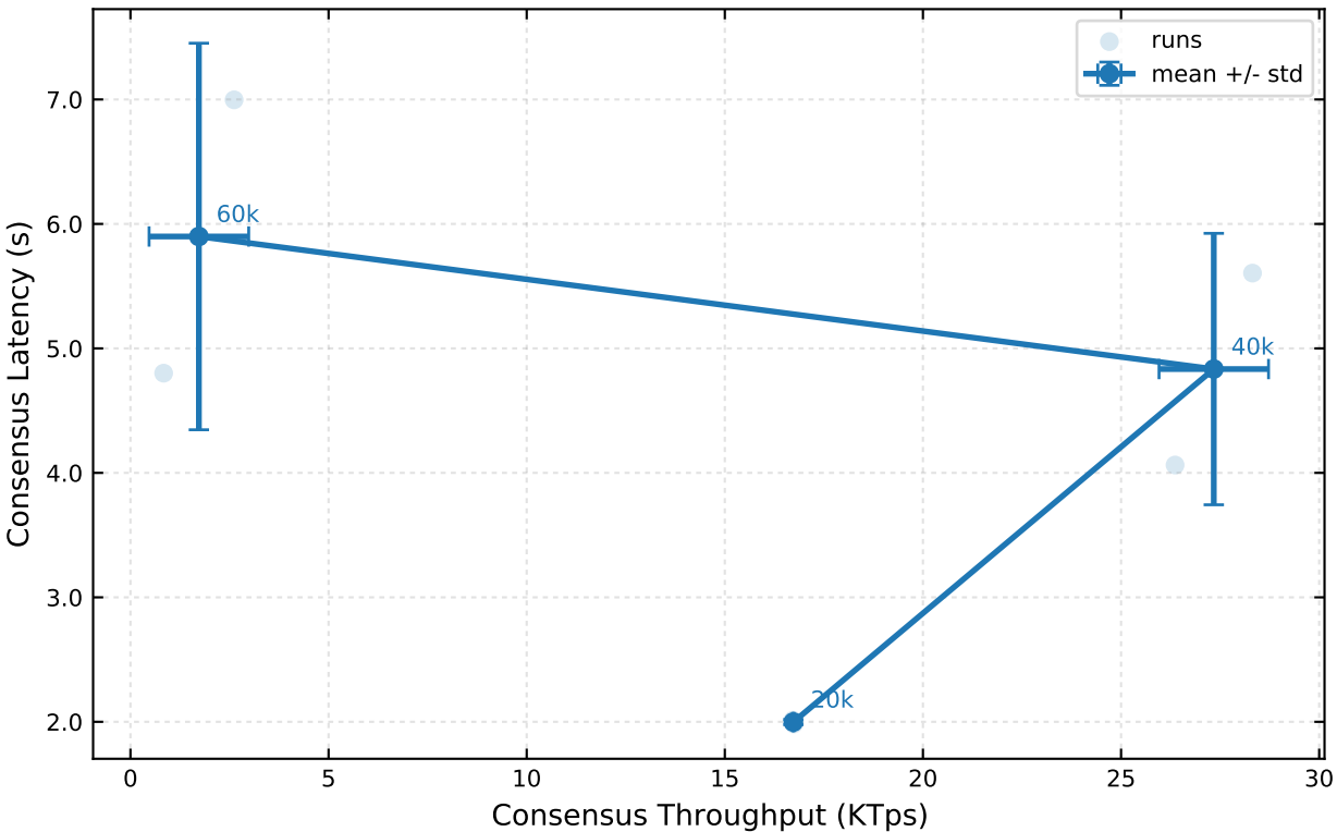
geo/old/custom-high-3 Consensus TPS-Latency
