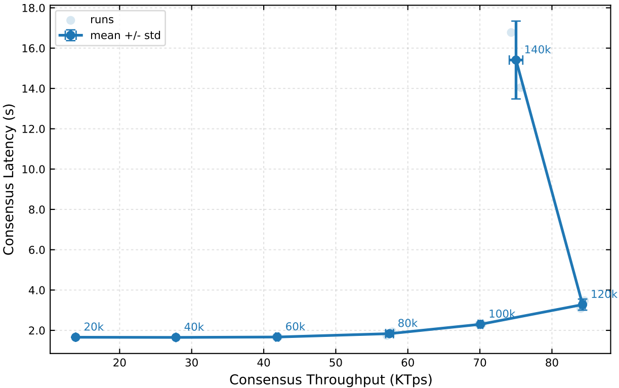
geo_uniform/balanced Consensus TPS-Latency
