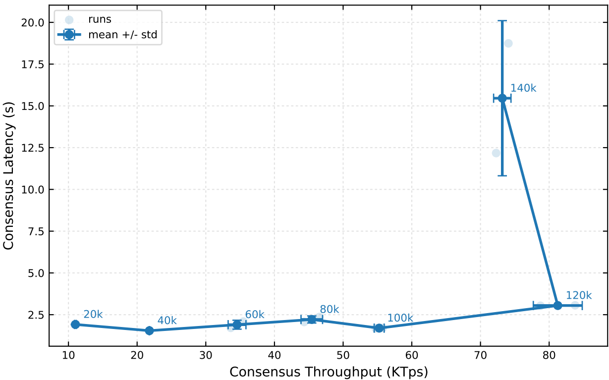
geo_uniform/custom-high-3 Consensus TPS-Latency
