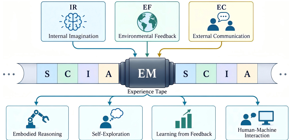
Figure 1: Overview of the Experience Machine. Different experience sources write state, critique, intent, and action sequentially onto a shared Experience Tape, enabling diverse experience-driven capabilities through the same underlying computation.
