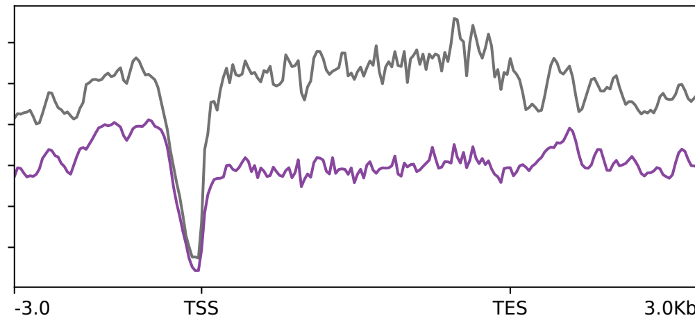
Hypomethylated
