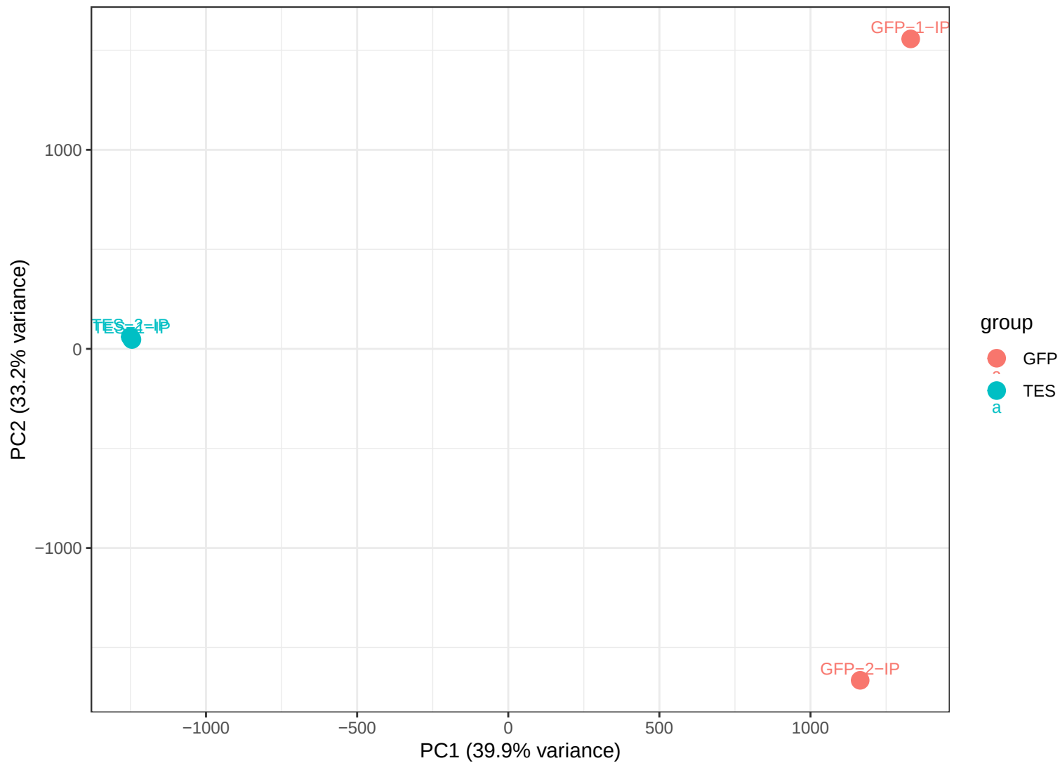
PCA of meDIP-seq Samples (INPUT Normalized Analysis)
