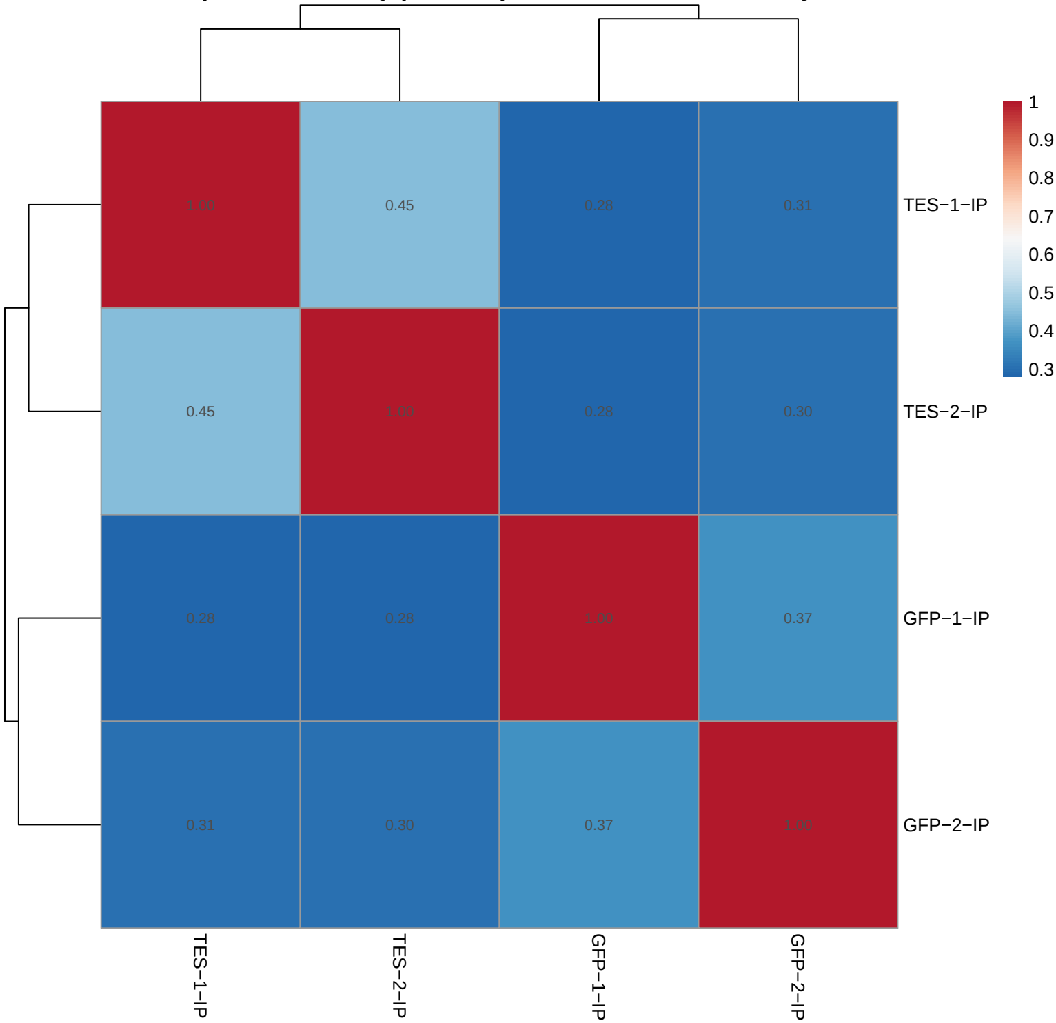
Sample Correlation (Spearman) – INPUT Normalized Analysis
