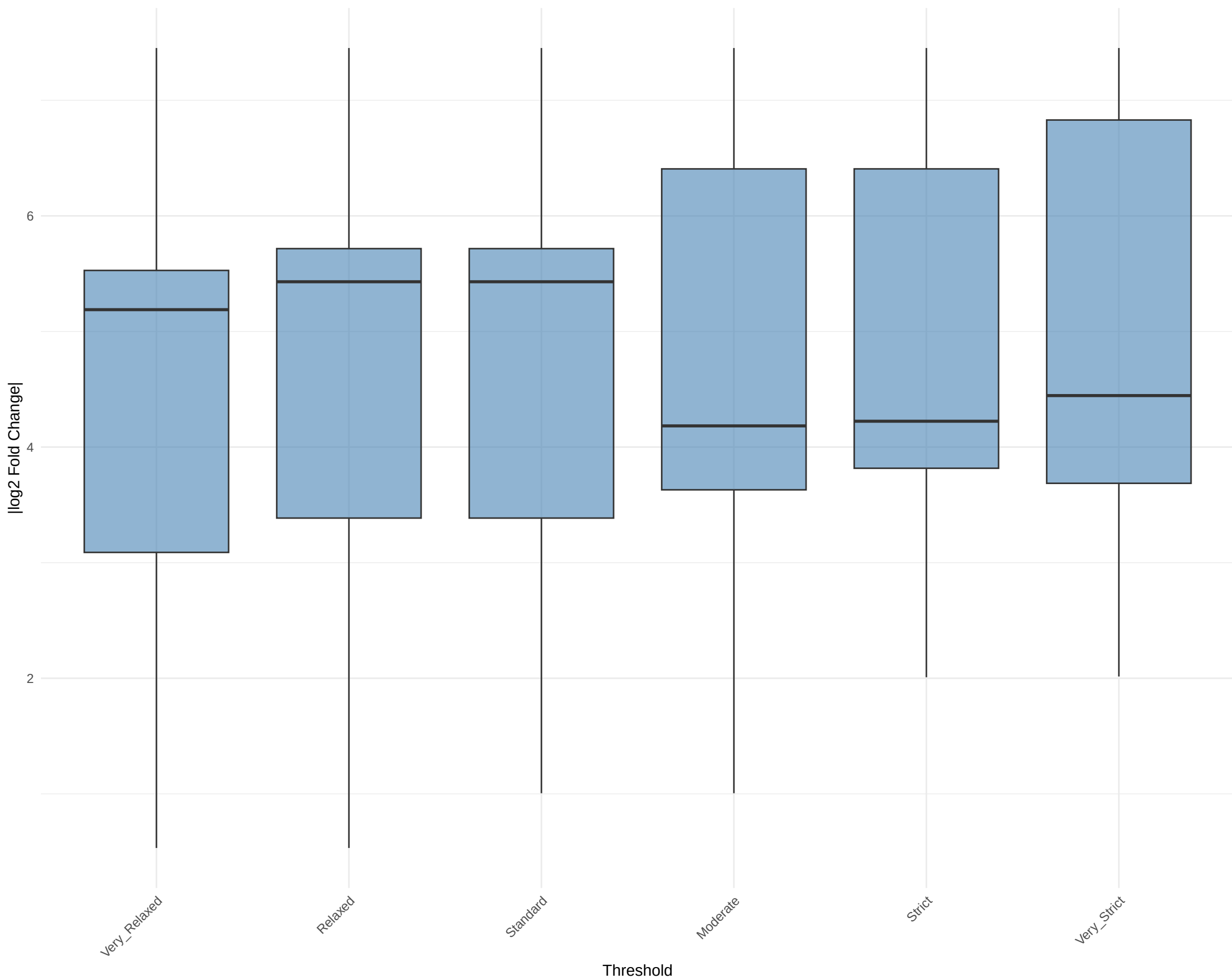
Effect Size Distribution by Threshold Stricter thresholds select for larger effect sizes
