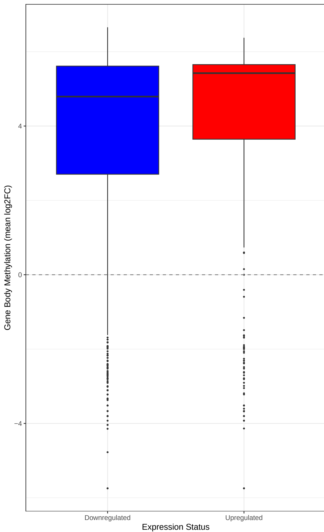
Gene Body Methylation by Expression Status
