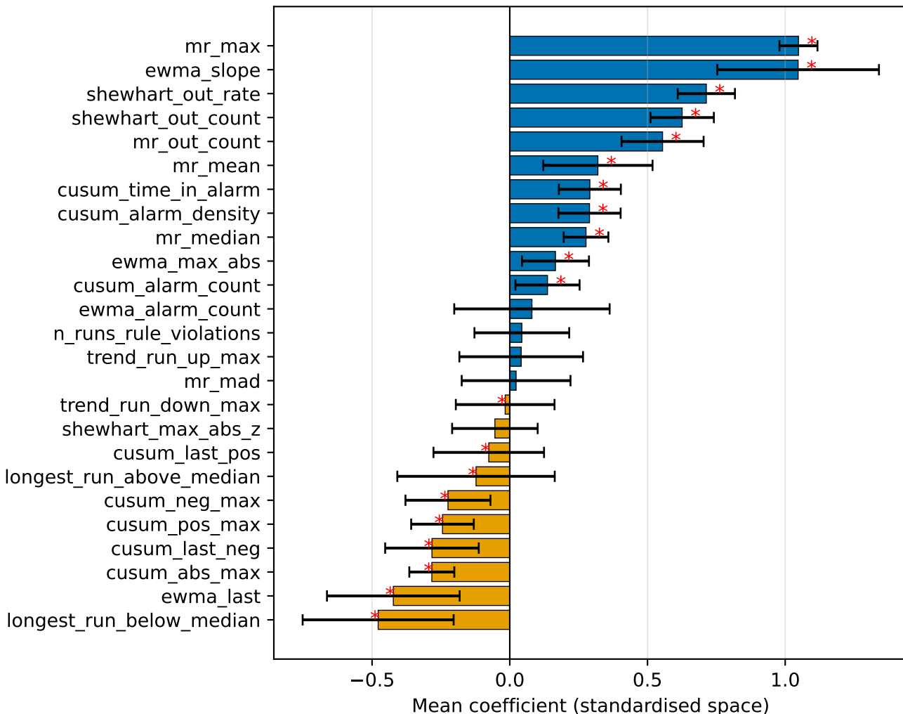
LogReg coefficients — B_SPC (* = stable sign, >80% or <20% folds positive)
