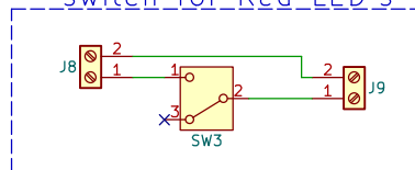
switch for Red LED's
