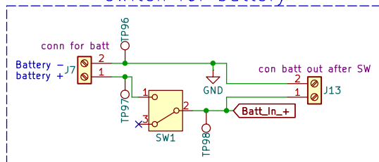
switch for battery
