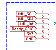
Header connectors for IMU
