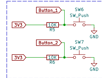
Push buttons
