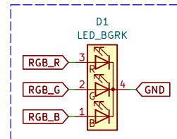
RGB LED
