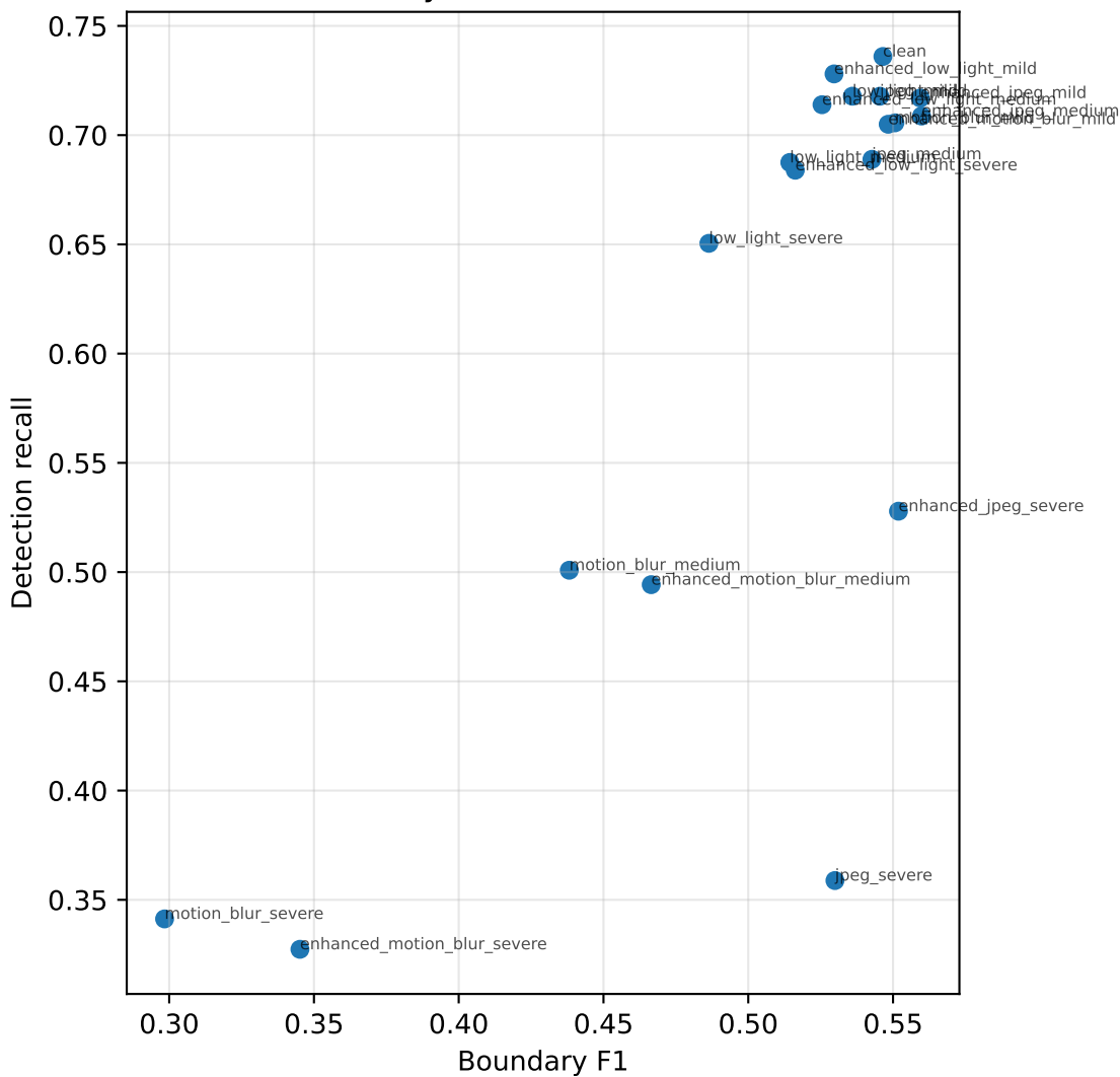
Boundary F1 vs detection recall
