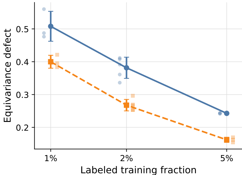
Equivariance defect
