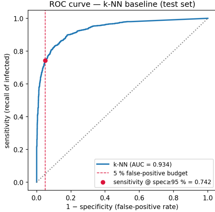
Figure 2: ROC curve of the k -NN baseline on the test set. The marked point corresponds to the competition metric — the highest sensitivity attainable at a specificity of at least 95 % (i.e. at most 5 % false alarms).
