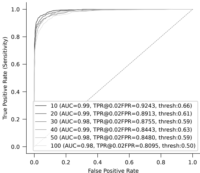
ROC Curve for Each Unique Suffix of Index (ratios \leq 100 )
