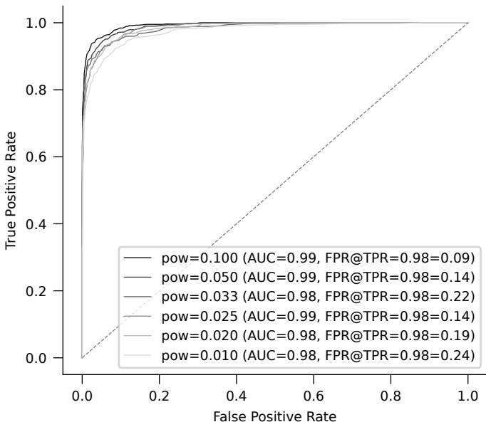
ROC by simulated mutation-detection power (ratios \leq 100 )
