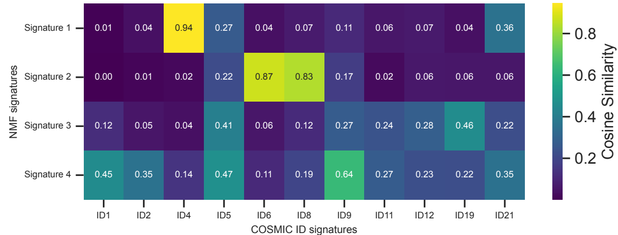
Cosine similarity: de novo ID signatures vs. COSMIC v3.4
