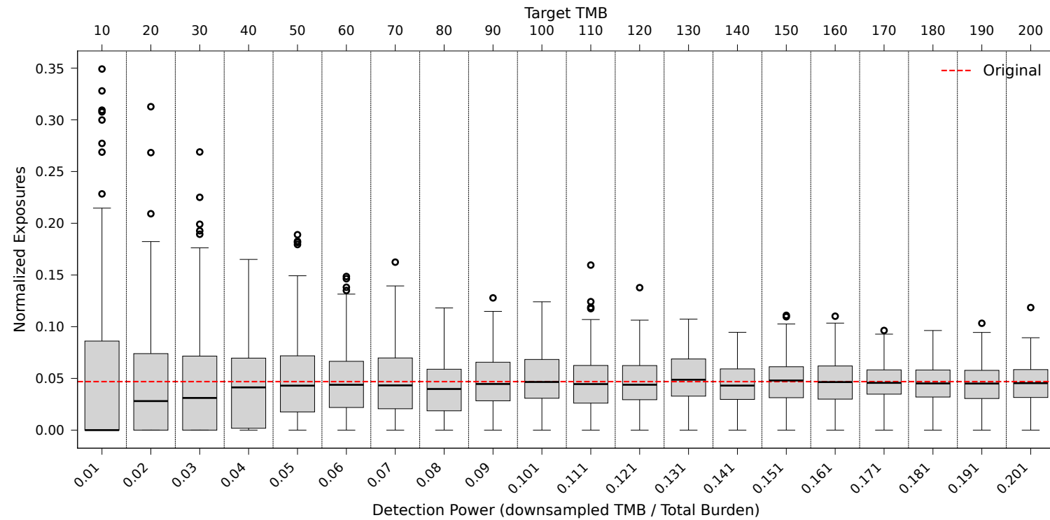
BTT4 trunk - SBS1 stability (nBoot=200)
