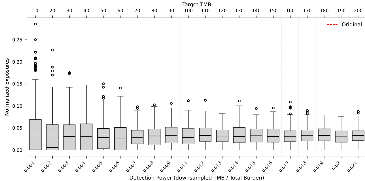
BTH4 trunk - SBS1 stability (nBoot=200)
