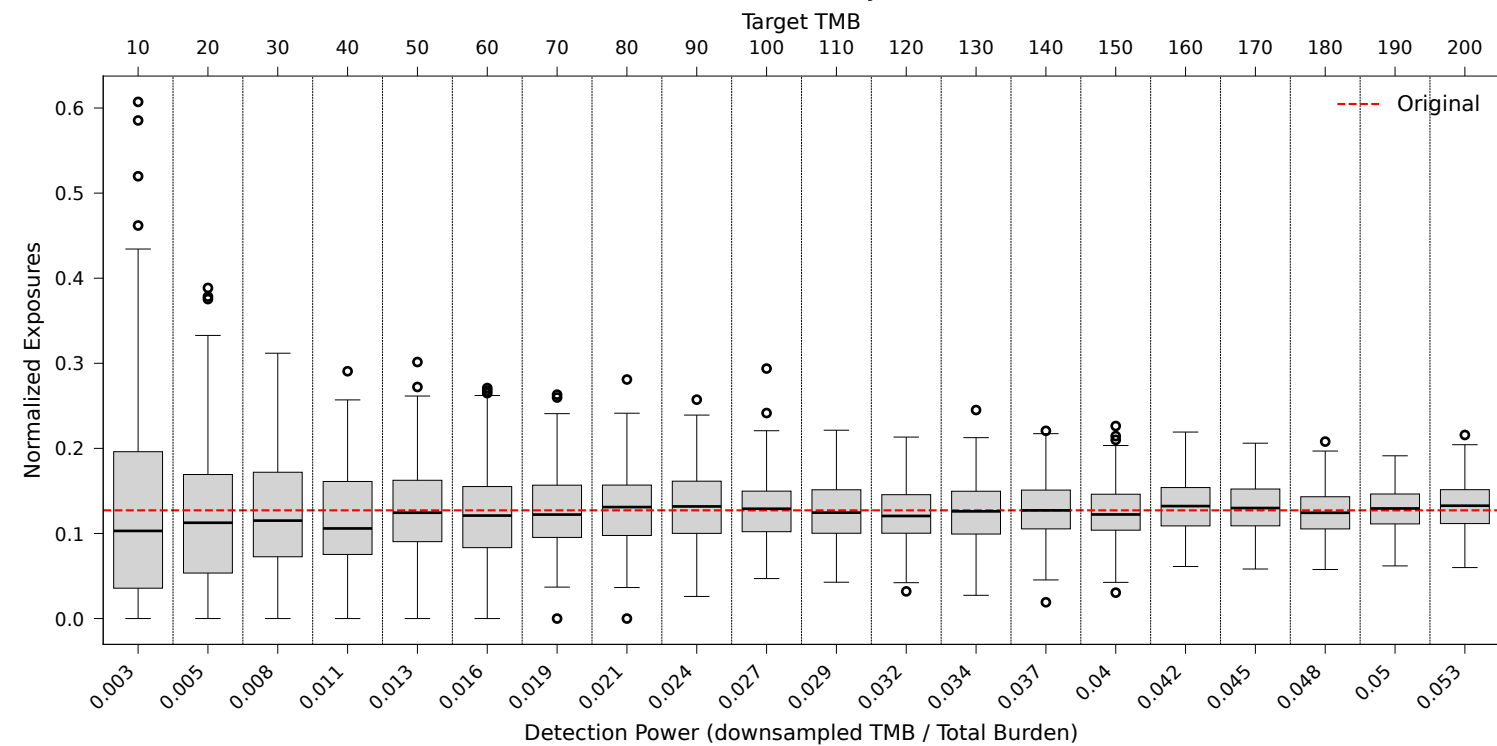
BTE4 trunk - SBS1 stability (nBoot=200)
