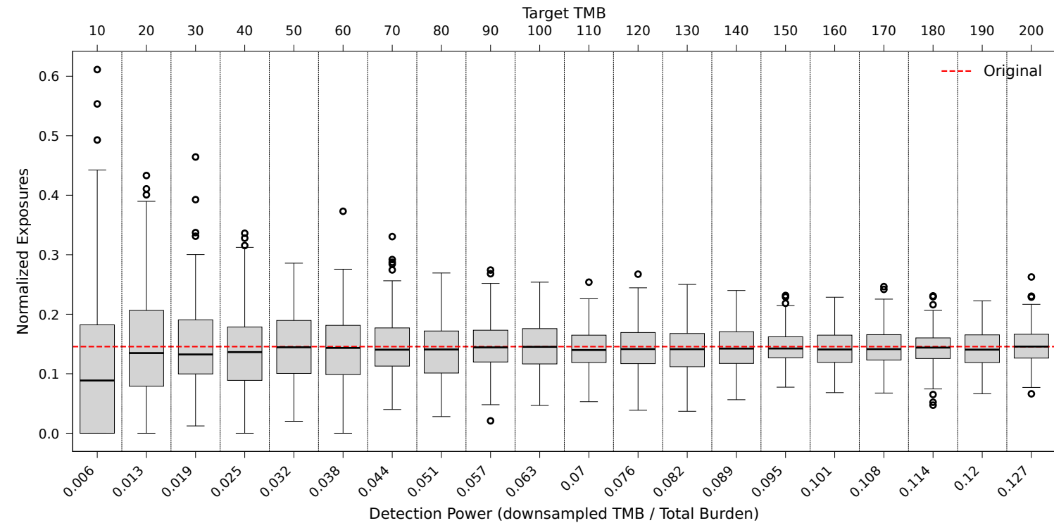
BTH5 trunk - SBS1 stability (nBoot=200)
