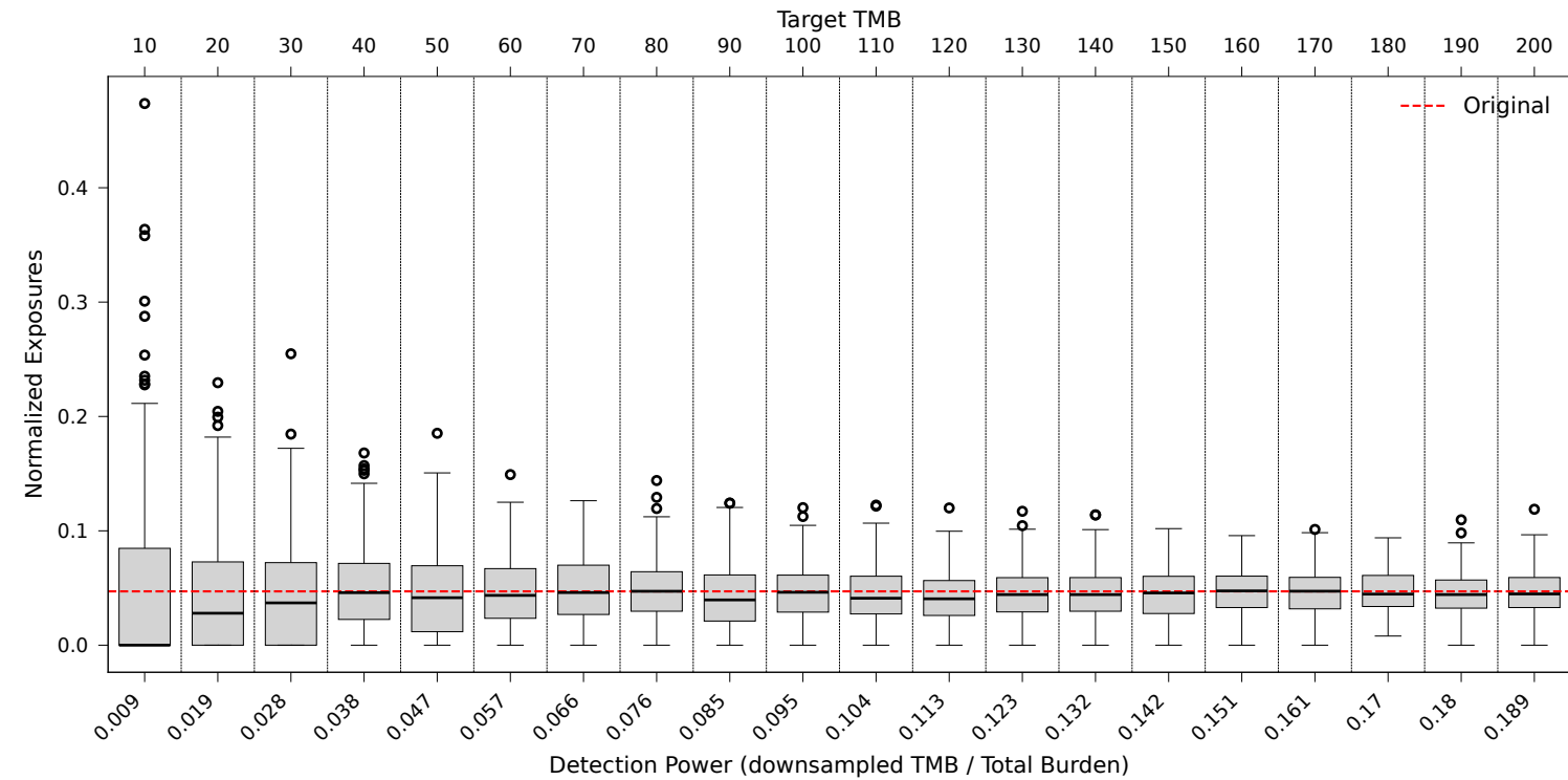
BTT7 trunk - SBS1 stability (nBoot=200)
