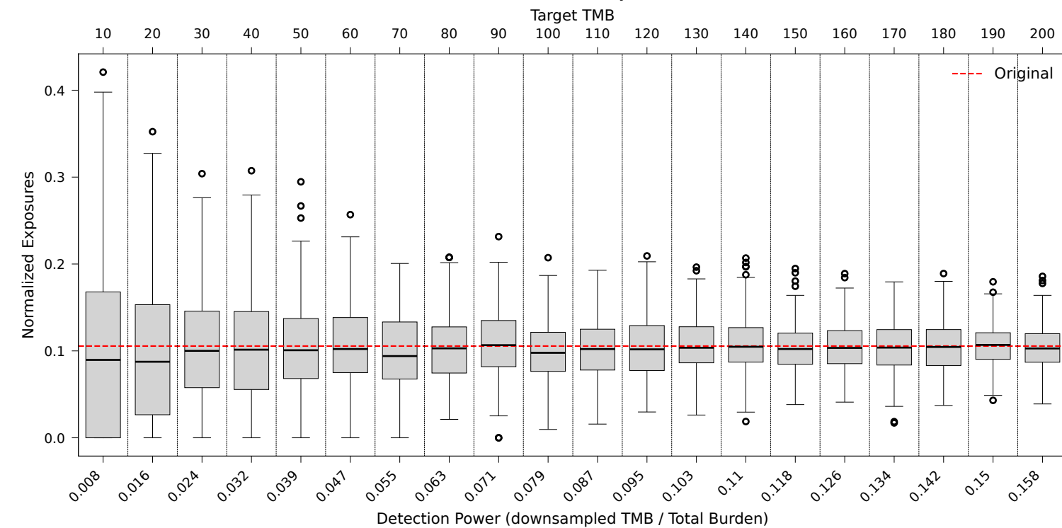
BTE1 trunk - SBS1 stability (nBoot=200)
