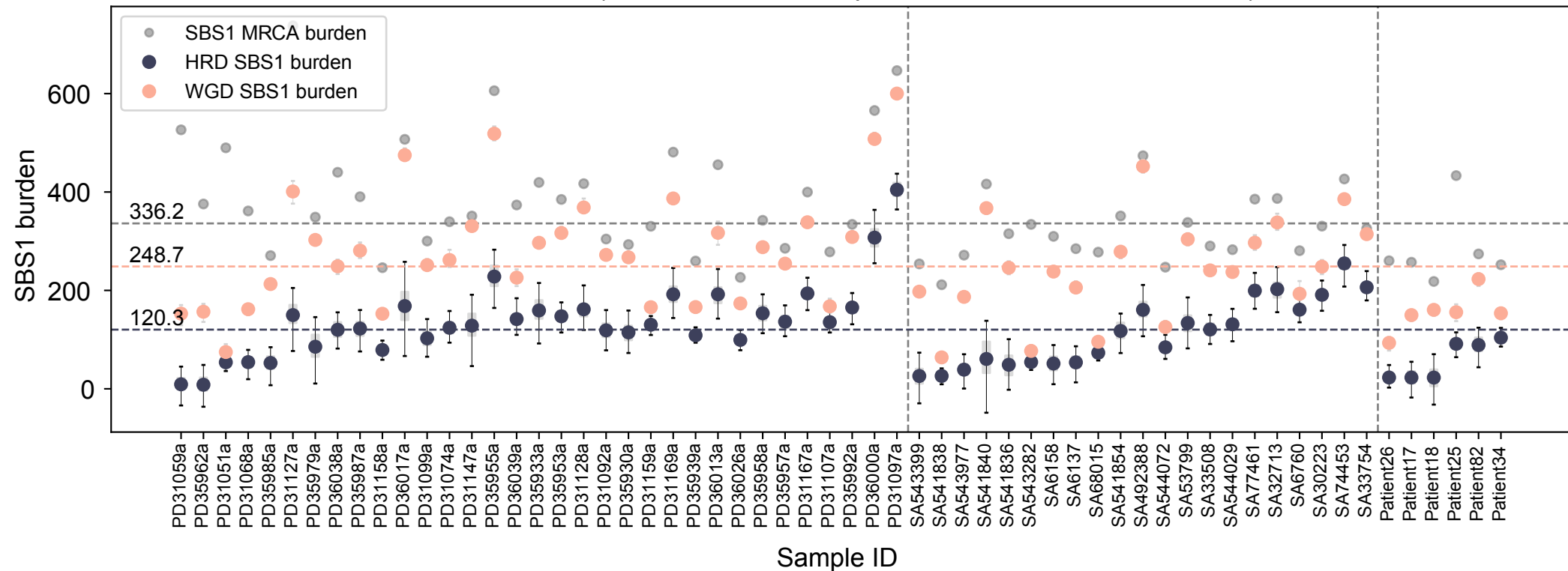
SBS1 Burden (Molecular Time \times Diploid-Genome–Corrected SBS1)
