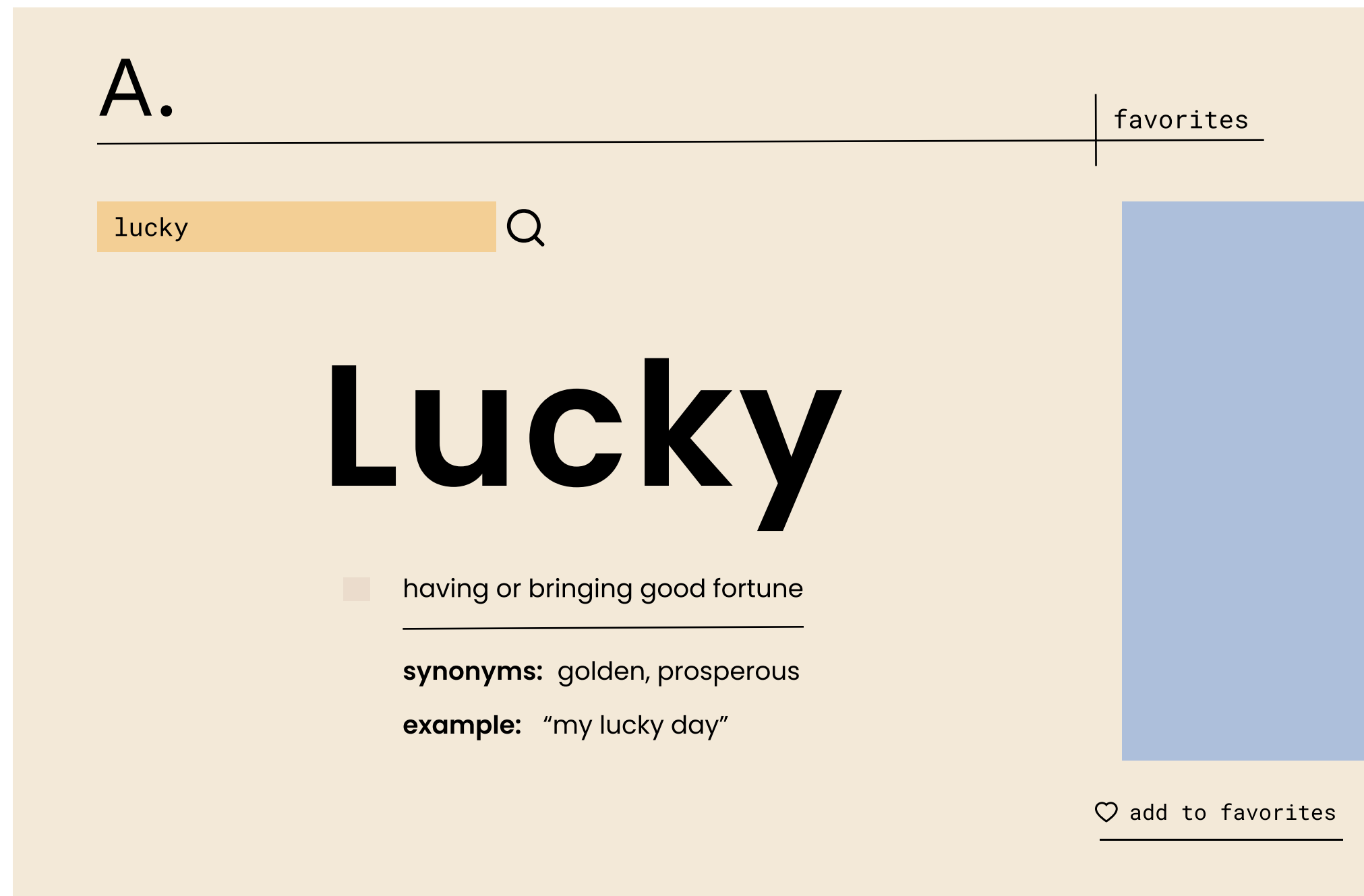
main page
