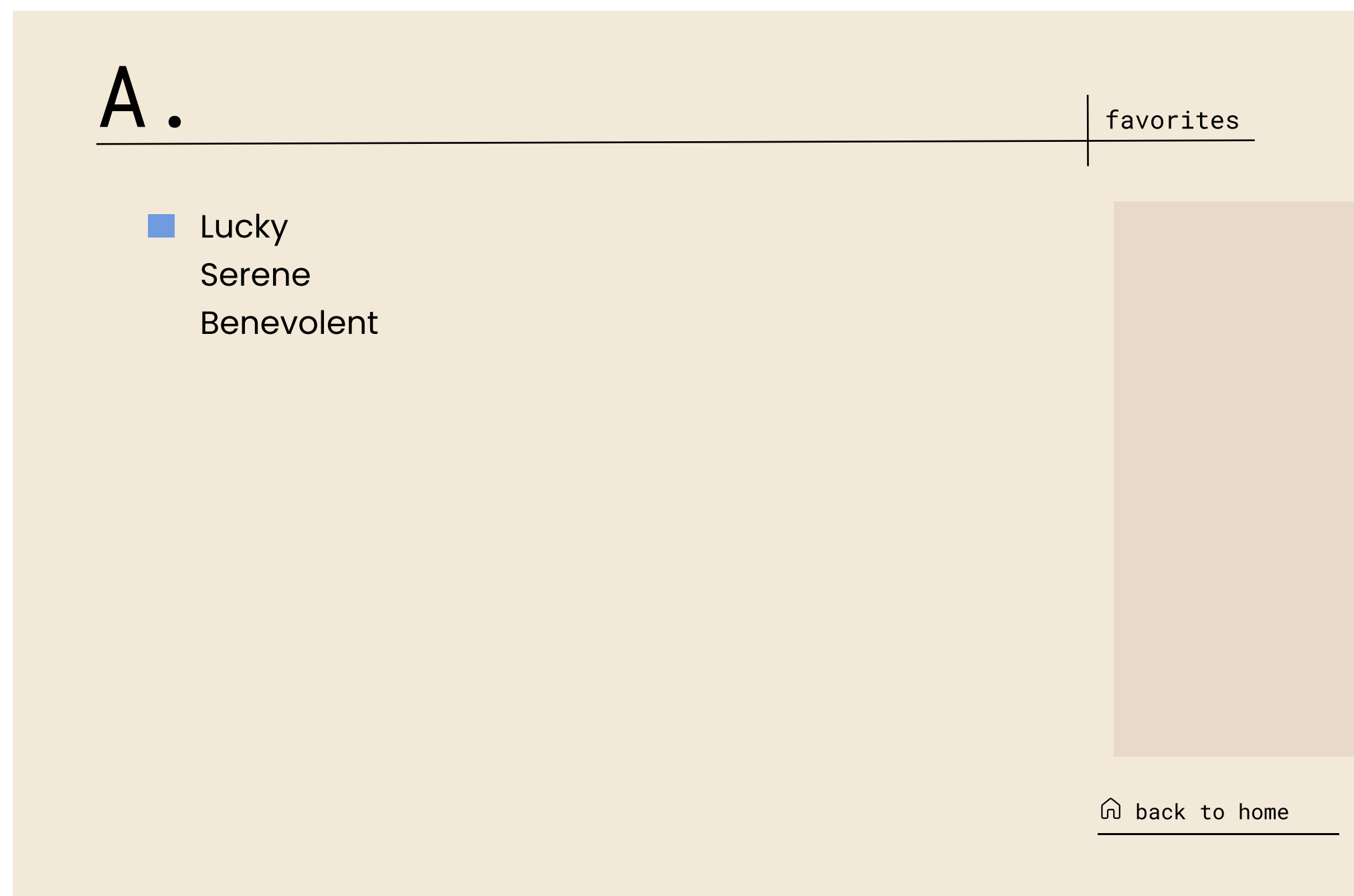
favorites page
