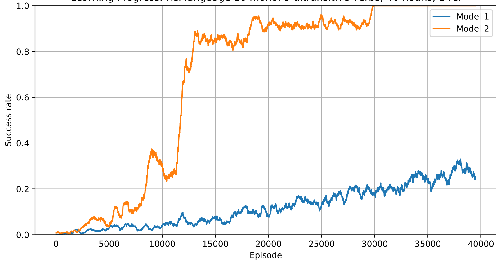
Learning Progress: Rel language 20 mono, 5 ditransitive verbs, 40 nouns, 1 rel
