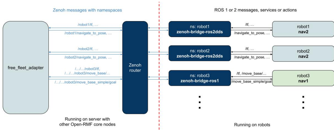
Figure 11.3: Free Fleet Adapter with Zenoh
