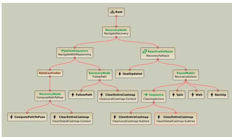
Figure 5.2: Humble Nav2 BT navigation navigate_to_pose_w_replanning_and_recovery.xml loaded with Groot2
