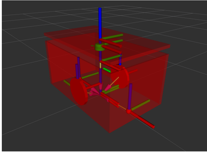
Figure 10.2: Jobot robot URDF model
