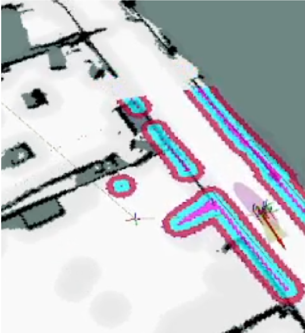
Figure 12.18: error when also AMCL fail
