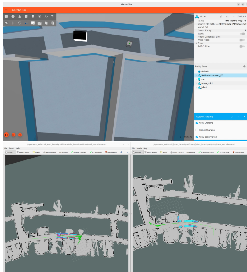
Figure 13.2: both robots simulated
