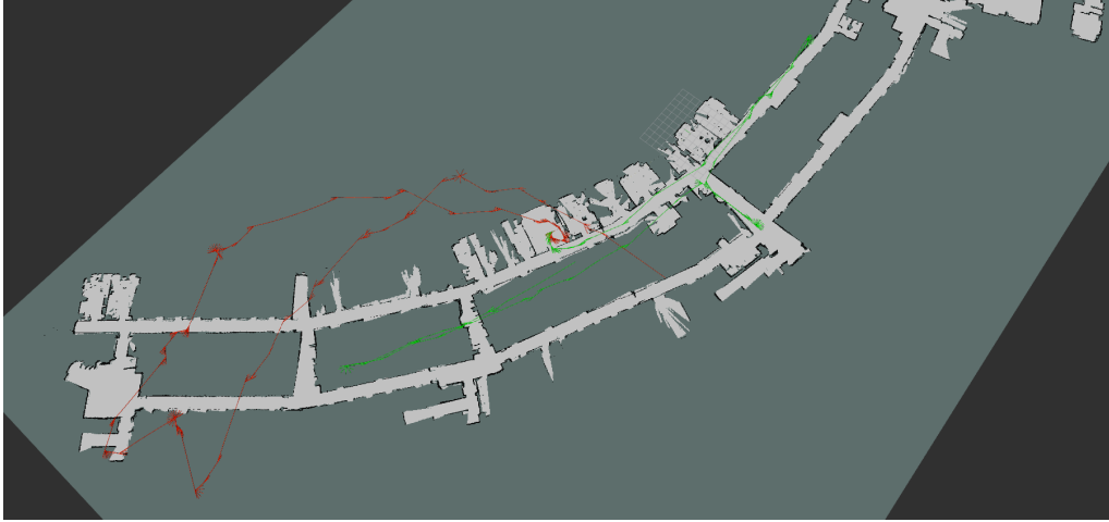
Figure 12.3: Mini odometry given by the robot (red) and odometry given by the robot_localization package (green)
