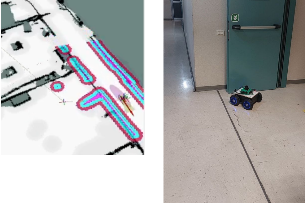
Figure 4.24: Examples when the estimation from AMCL fails
