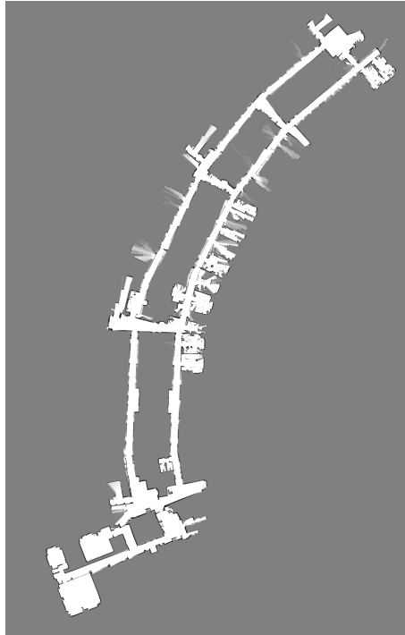
Figure 9.2: Map acquired with Cartographer
