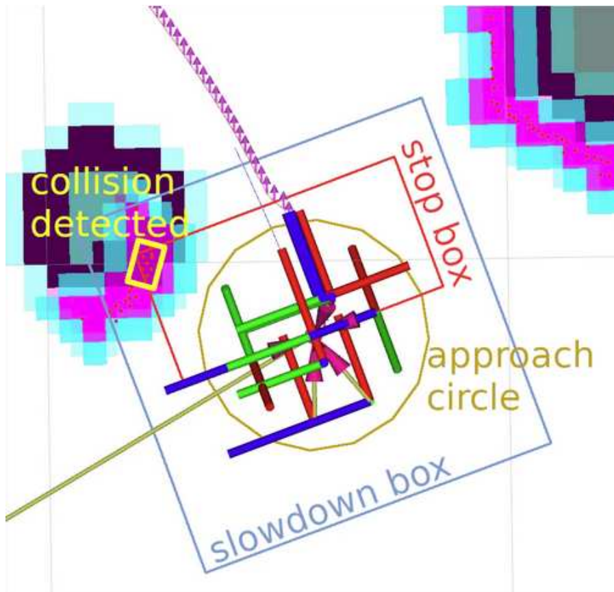
Figure 4.27: Collision monitor control boxes
