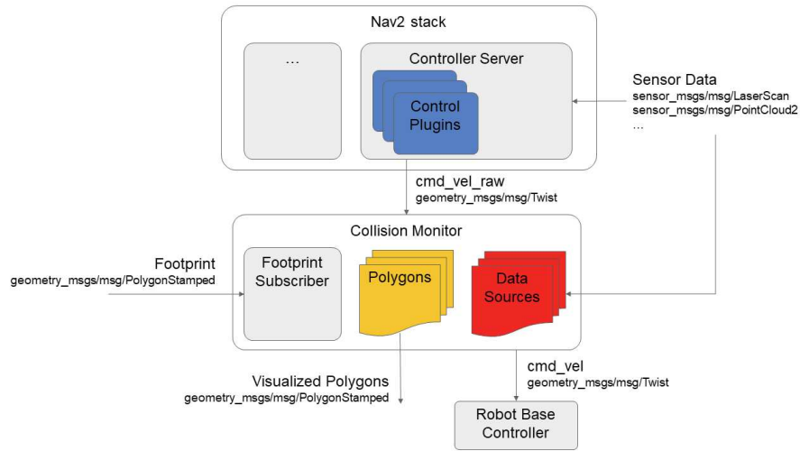
Figure 4.26: Collision monitor diagram
