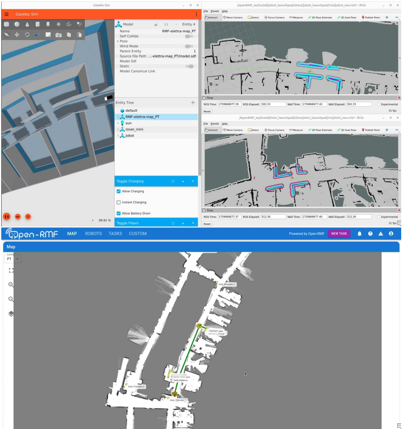
Figure 5.3: images navigation of the 2 robots with open-rmf in simulated environment
