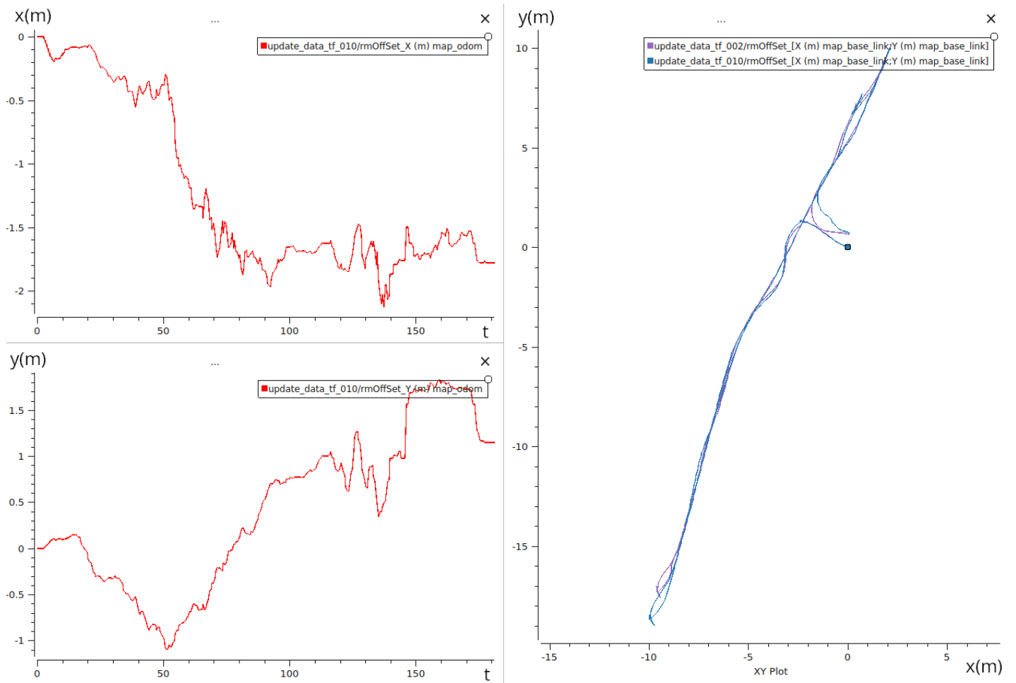
Figure 4.18: On the left the correction in position performed by AMCL; on the right the path corrected by AMCL
