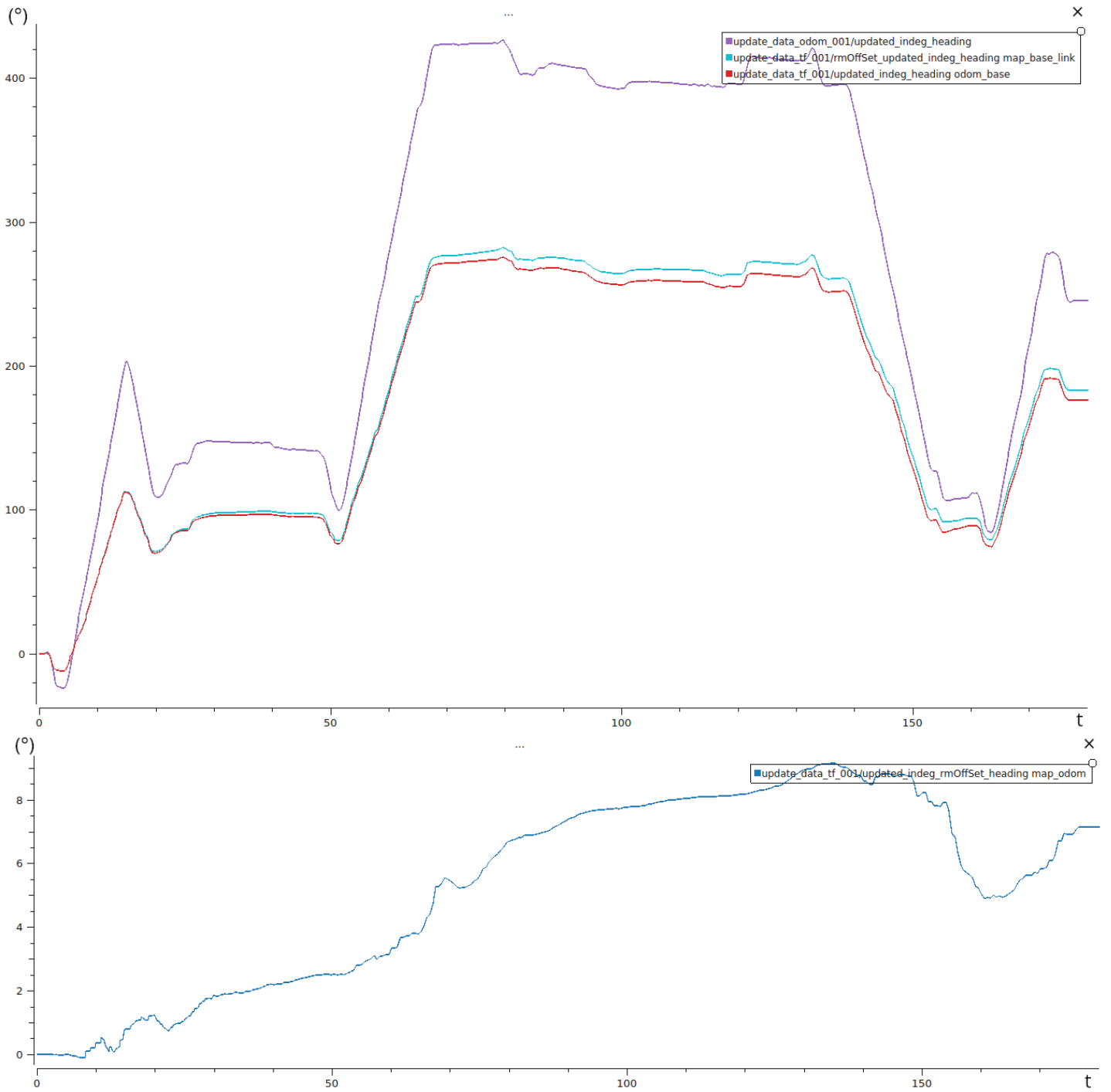
Figure 4.16: On top heading values returned by the system; down the heading correction for the Mini performed by AMCL
